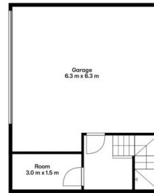
Basement
