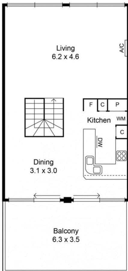
Upper Level
