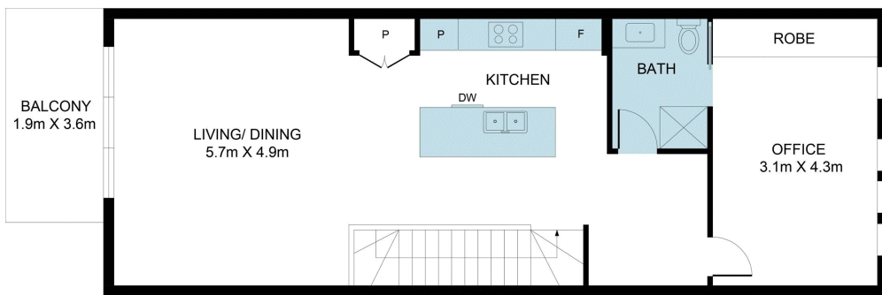
GROUND FLOOR
