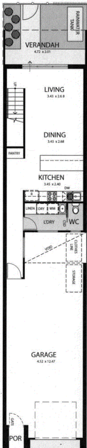
GROUND FLOOR
