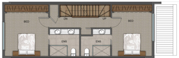
First Floor
